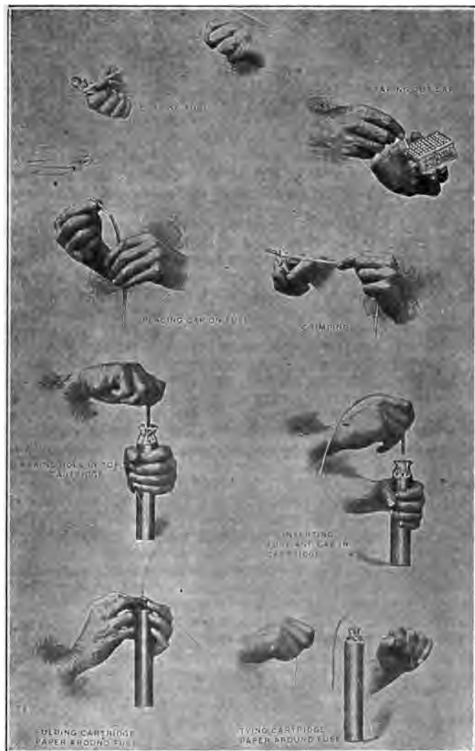
Fig. 90. Priming With a Fuse Cap (Du Pont).
